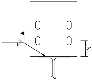
TYPICAL AT 8" MEMBERS
