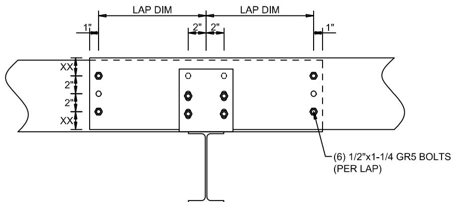
STANDARD LAP DETAIL
