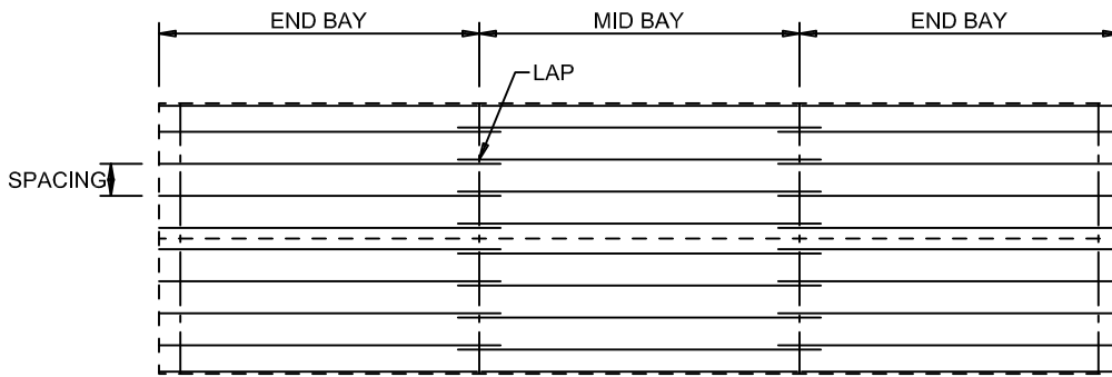
3+ BAY BUILDING
