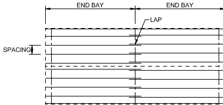
2 BAY BUILDING
